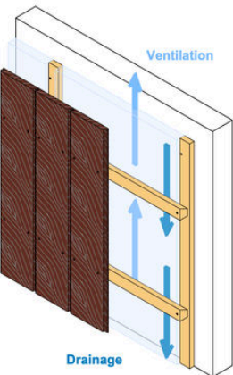
○ Typical indicative cladding wall build up.
